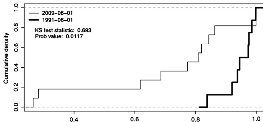
Fig. 3. Empirical cumulative distribution of R^2 .
